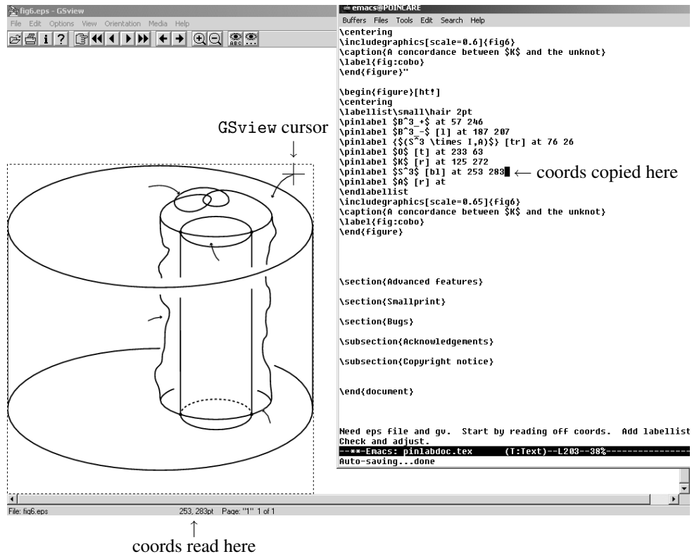
Figure 2: Screenshot
